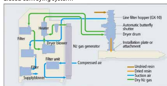
Closed conveying system
